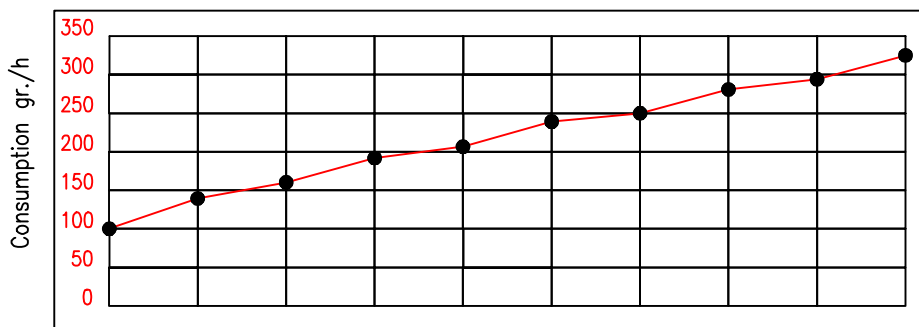
Catalytic Panel S/2000 – L.P.G. gas Consumption/Thermic power/Gas pressure ratio
